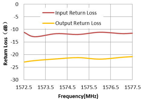
Return Loss
