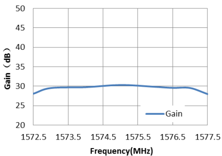
Gain
