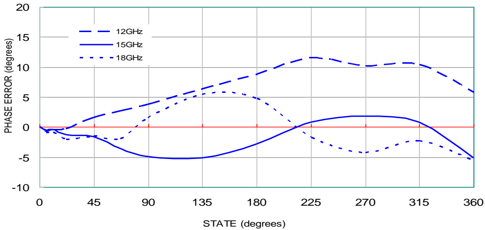
Phase Error vs. State
